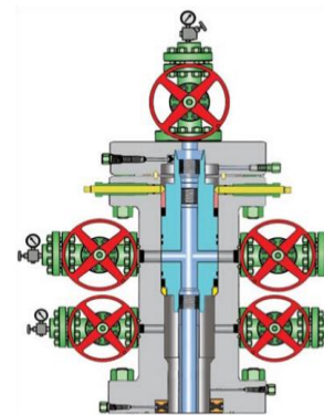
Integrated compact wellhead and horizontal tree
